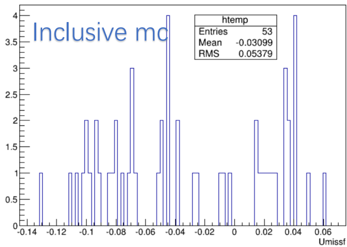
Umissf {BDT>0.23}
