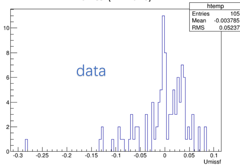
Umissf {BDT>0.23}
