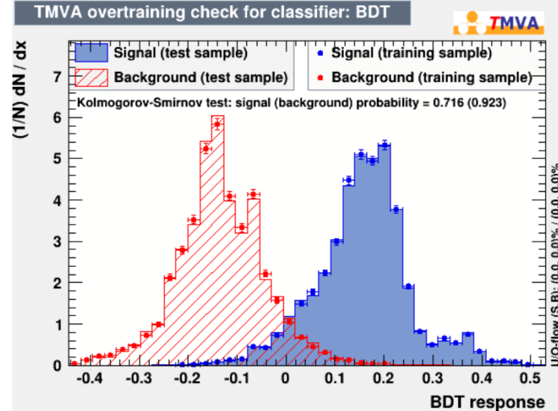
Training data
