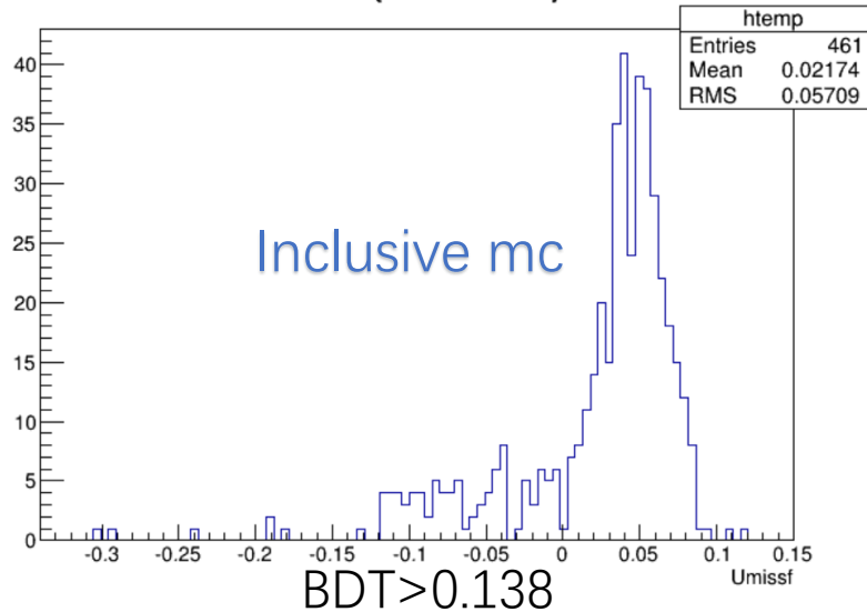
Umissf {BDT>0.1380}
