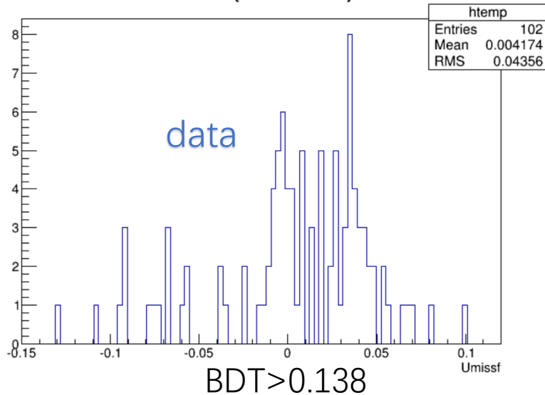
Umissf {BDT>0.1380}
