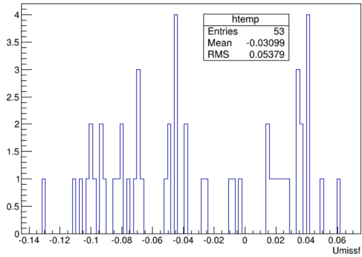
Inclusive mc
