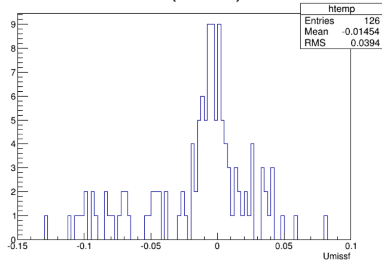
mixture
