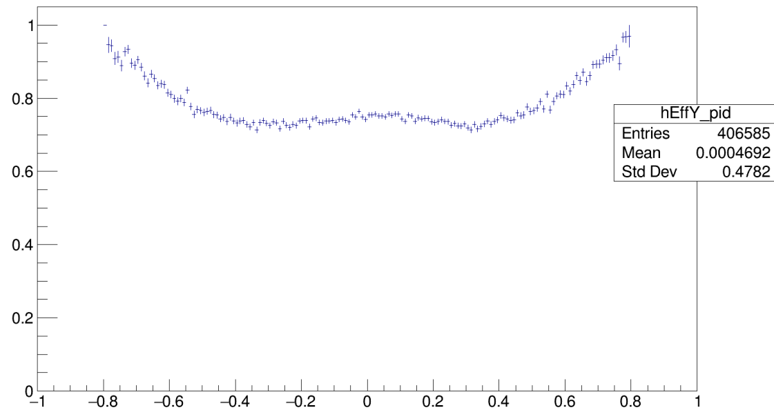
Rapidity eff distribution of the mother (443), accepted PID
