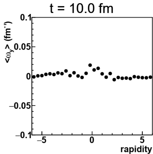
Parton local vorticity depend on rapidity
